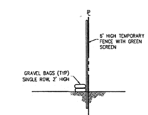
2 TEMPORARY FENCING DETAIL NTS
