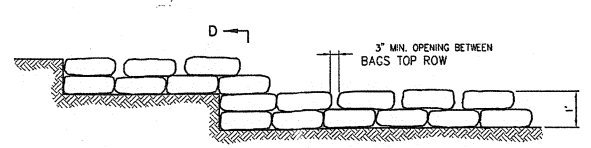
1 TYPICAL GRAVELBAG DETAIL
