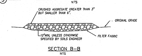
3 STABILIZED CONSTRUCTION ENTRANCE/EXIT DETAIL (TYPE 2) NTS
