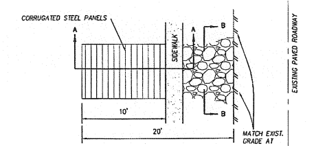
3 STABILIZED CONSTRUCTION ENTRANCE/EXIT DETAIL (TYPE 2) NTS
